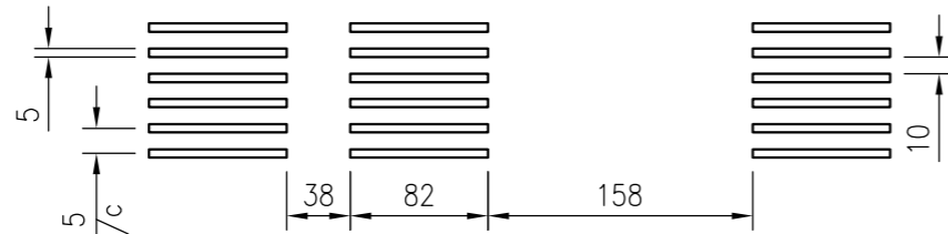
① Perforation Detail SCALE 1:5
