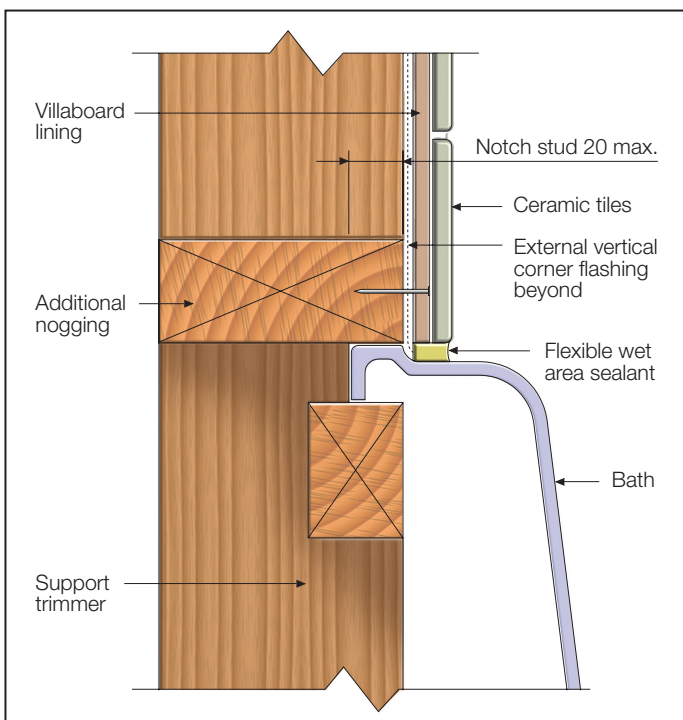
FIGURE 24 BATH EDGE DETAIL - VILLABOARD LINING TO BE FINISHED WITH TILES
