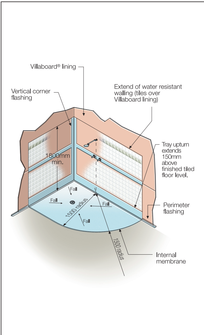
FIGURE 20 UNENCLOSED SHOWERS
