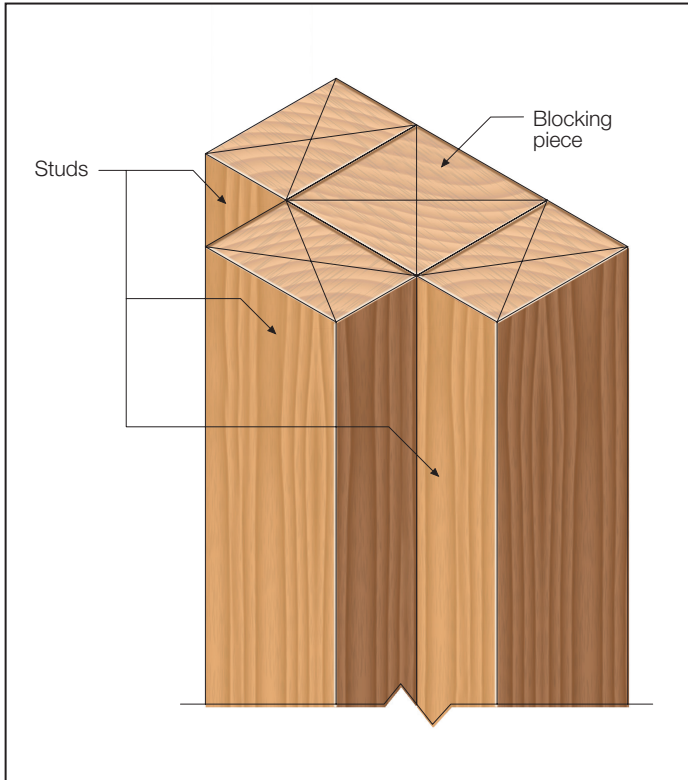
FIGURE 2 BLOCKED CORNER
