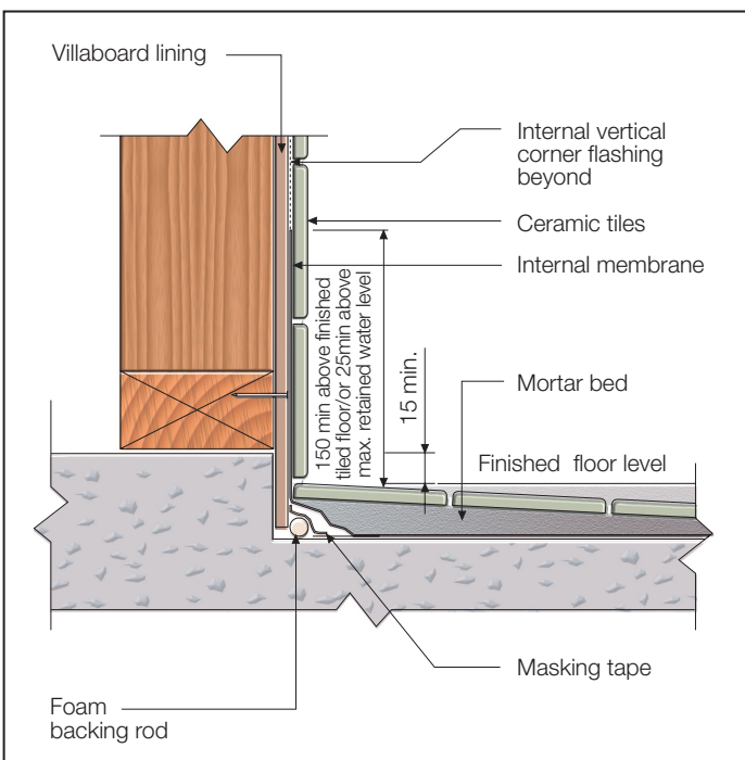
FIGURE 15 IN-SITU APPLIED INTERNAL MEMBRANE AT STEP-DOWN
