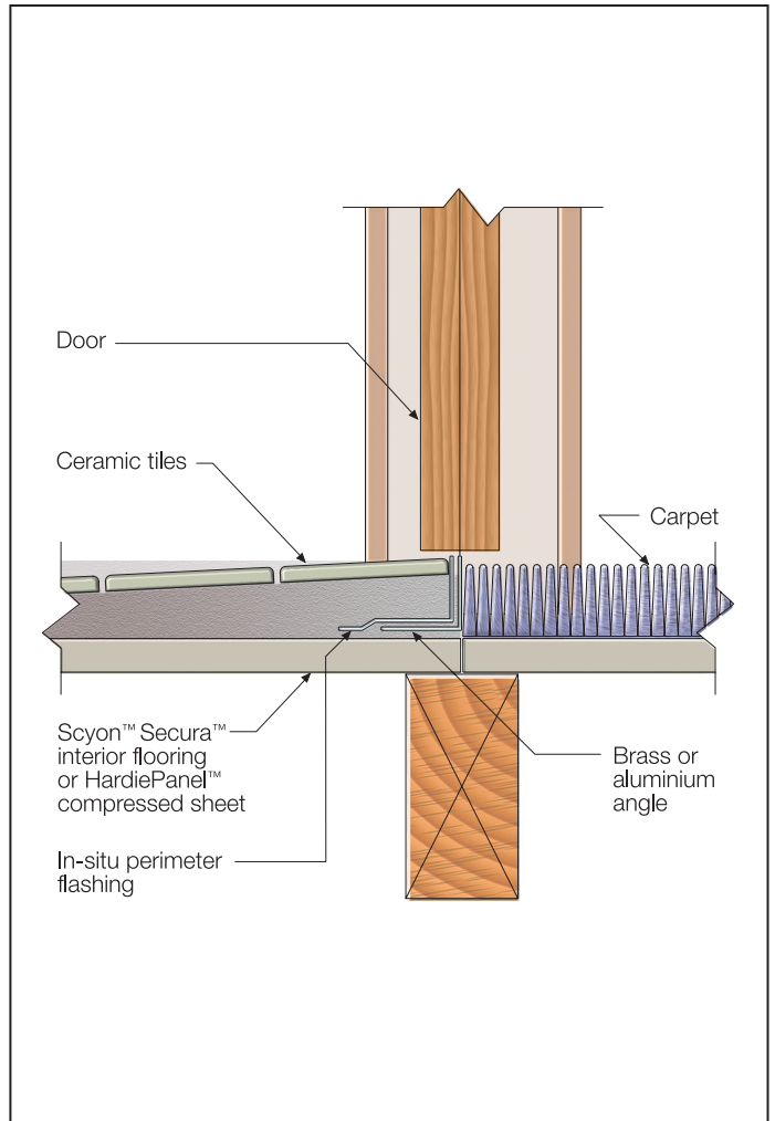
FIGURE 8 DOORWAY FLASHING
