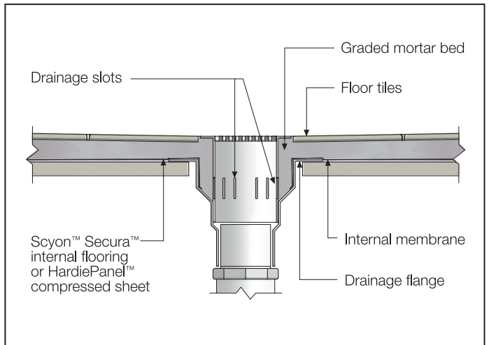
FIGURE 27 PRINCIPLE OF LEAK CONTROL WASTE
