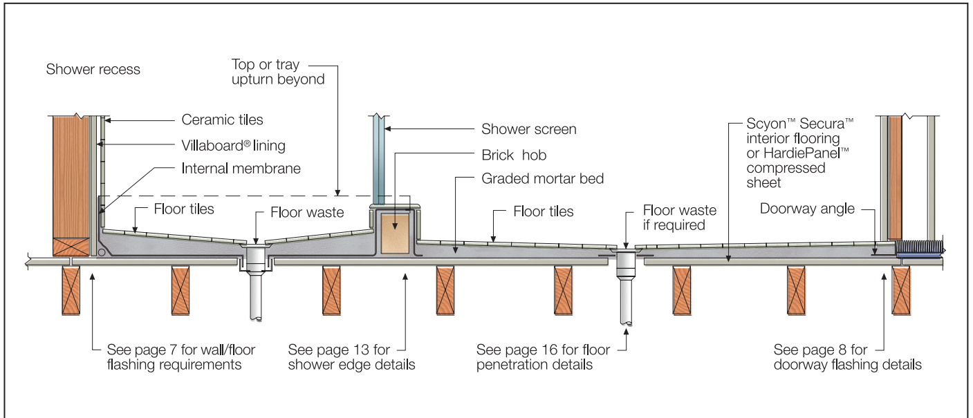
FIGURE 1 TYPICAL BATHROOM CROSS-SECTION
