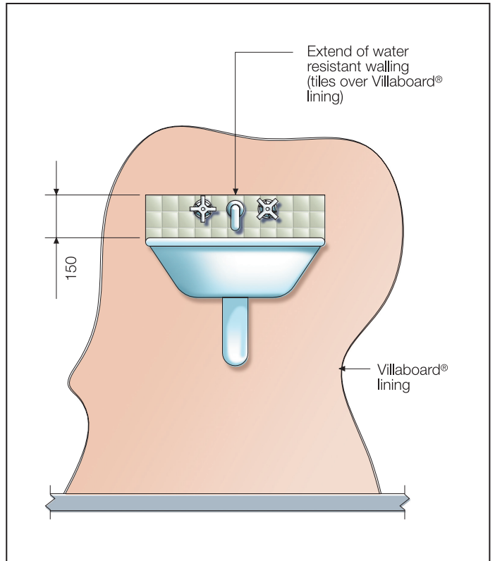
FIGURE 25 WATERPROOFING VESSELS ABUTTING WALLS
