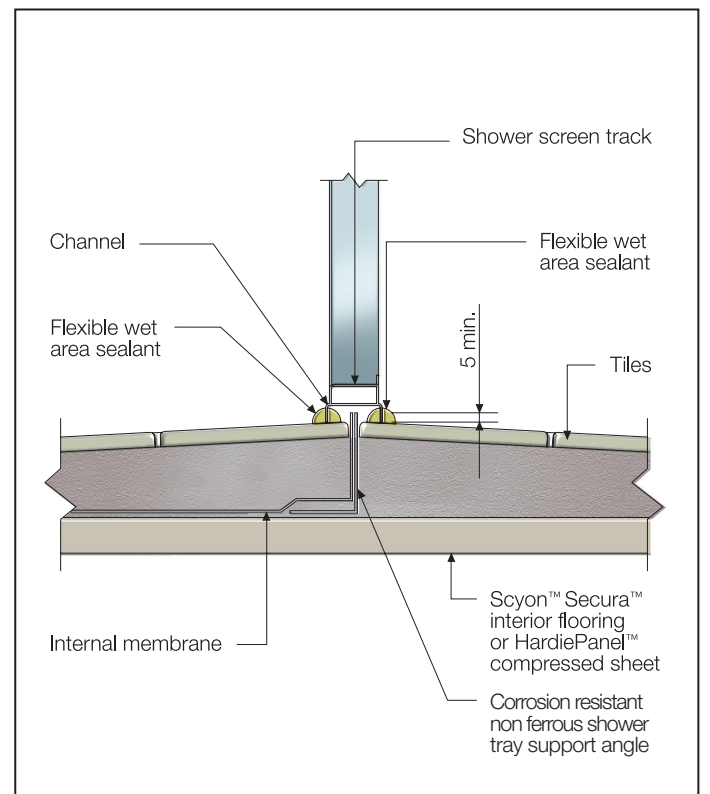
FIGURE 19 HOBLESS SHOWER
