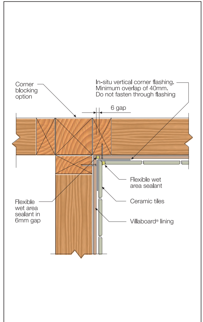
FIGURE 10 VERTICAL CORNER FLASHING FOR INTERNAL MEMBRANE - SHOWER RECESS
