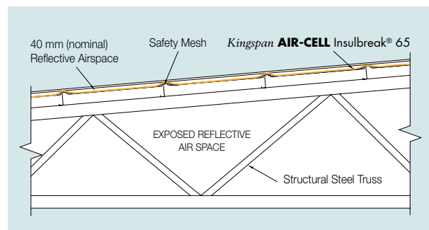
Figure 8 Side elevation of Kingspan AIR-CELL Insulbreak® 65 in a commercial warehouse
