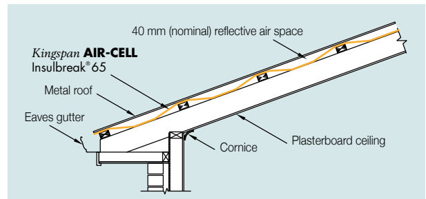
Figure 4 Side elevation of Kingspan AIR-CELL Insulbreak® 65 in a metal roof with a raked ceiling
