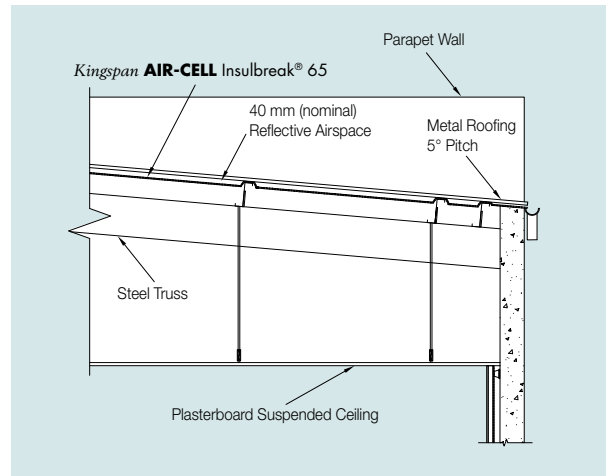
Figure 7 Side elevation of Kingspan AIR-CELL Insulbreak® 65 in a commercial office
