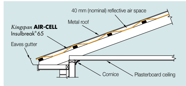
Figure 3 Side elevation of Kingspan AIR-CELL Insulbreak® 65 in a metal roof with a flat ceiling
